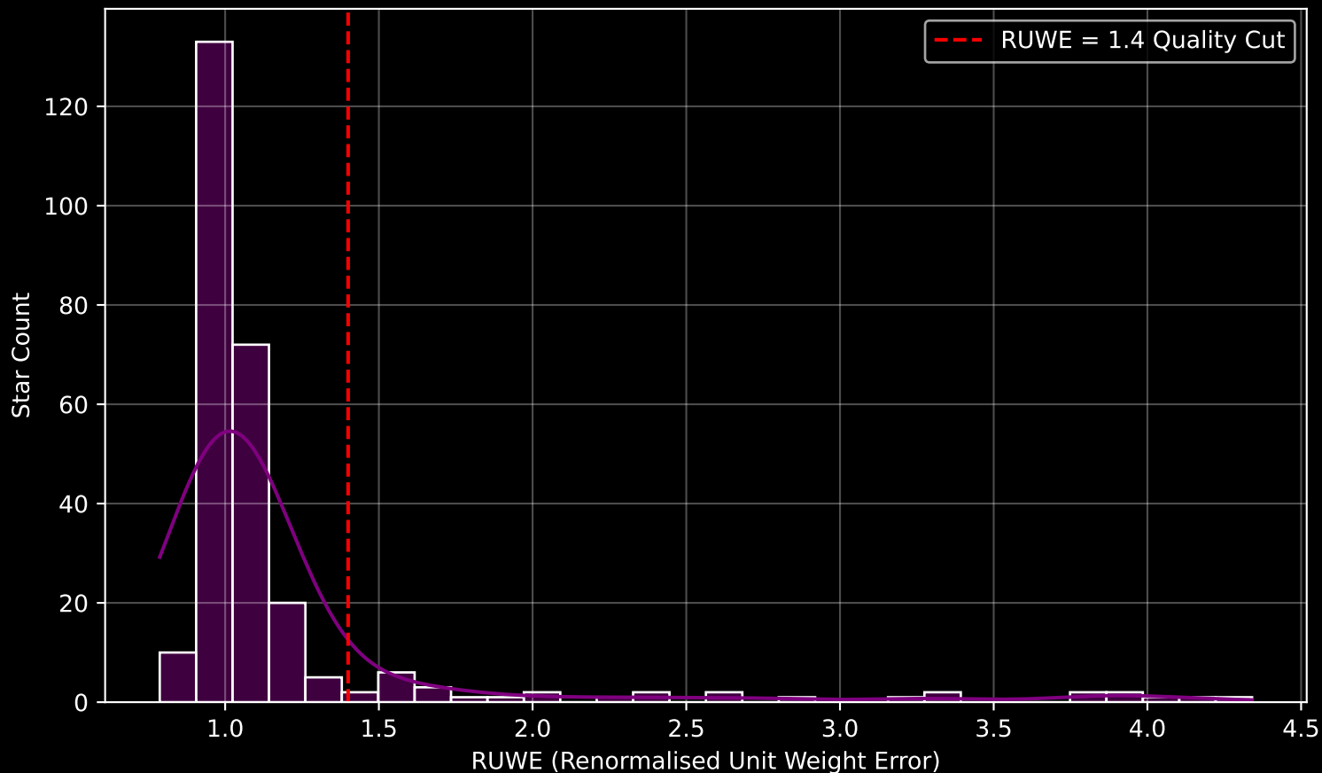
GALAH DR4 Field [6925] RUWE Distribution (n= 271)
