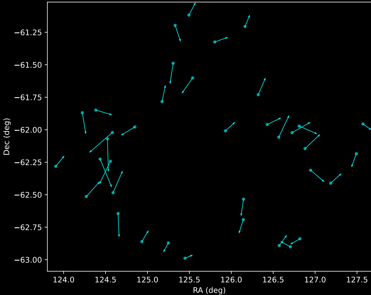
GALAH DR4 Noise Stream Proper Motion Vectors (n=37)
