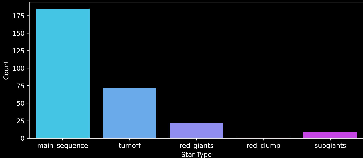
GALAH DR4 Field: [6925] Count plot of Star Type
