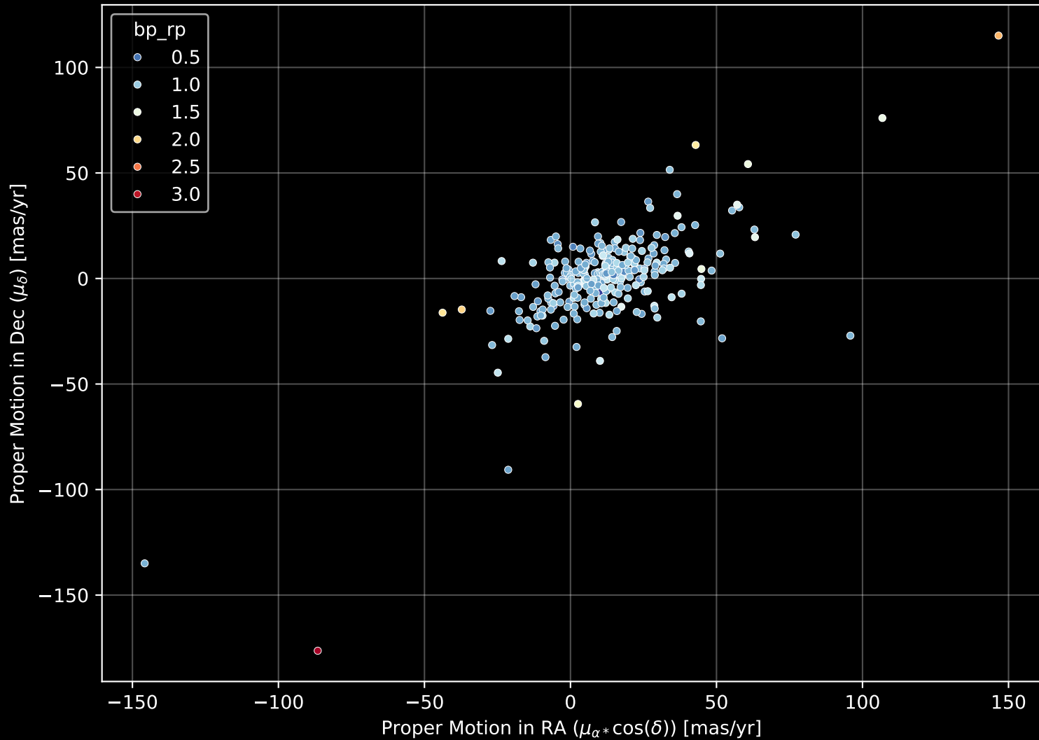
GALAH DR4 Field: [6925] Proper Motion Diagram (n= 288)
