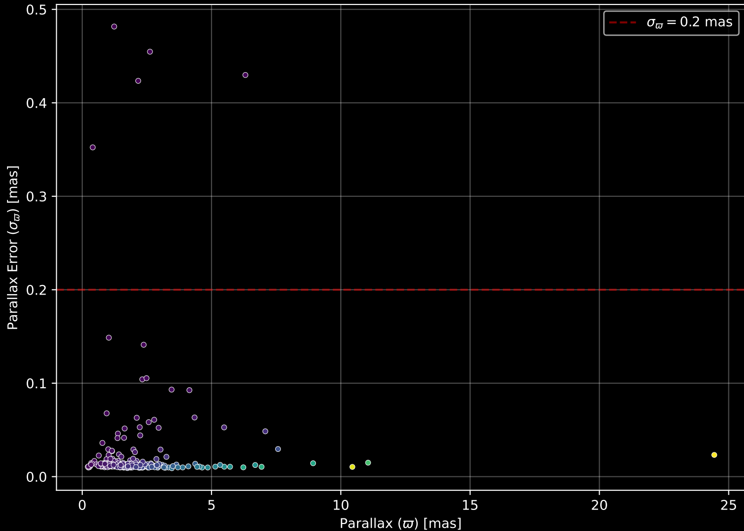
GALAH DR4 Field: [6925] Parallax Quality (n= 288)
