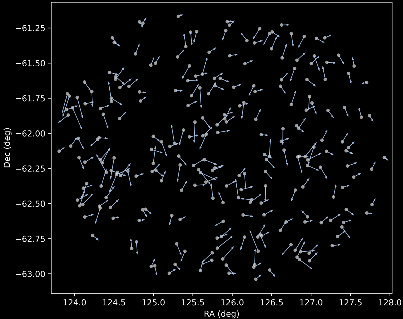
GALAH DR4 Cluster 1 Proper Motion Vectors (n=246)
